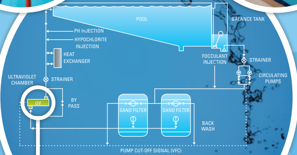
Flow Diagram for Single Pool with Ultraviolet Disinfection
